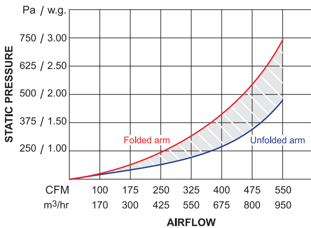
OSKAR FUME ARM Ø125
