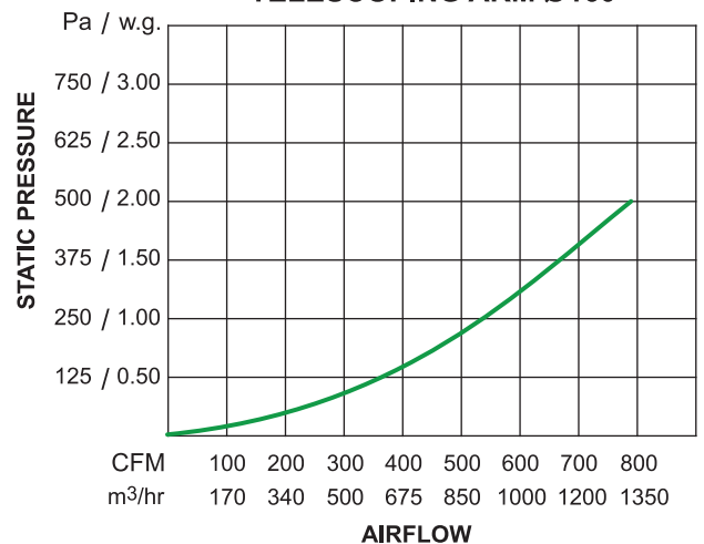
TELESCOPING ARM Ø160
